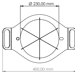
76587 Manual Watermelon Cutting Tool Blade (6 Pieces) (Assembled)
