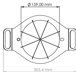
76505 Manual Melon Cutting Tool Blade (8 Pieces) (Assembled)
