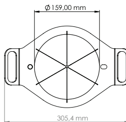
76507 Manual Melon Cutting Tool Blade (6 Pieces) (Assembled)
