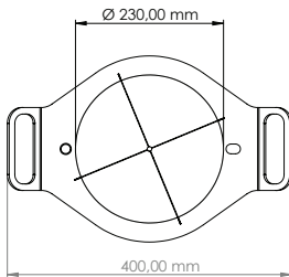
76586 Manual Watermelon Cutting Tool Blade (4 Pieces) (Assembled)
